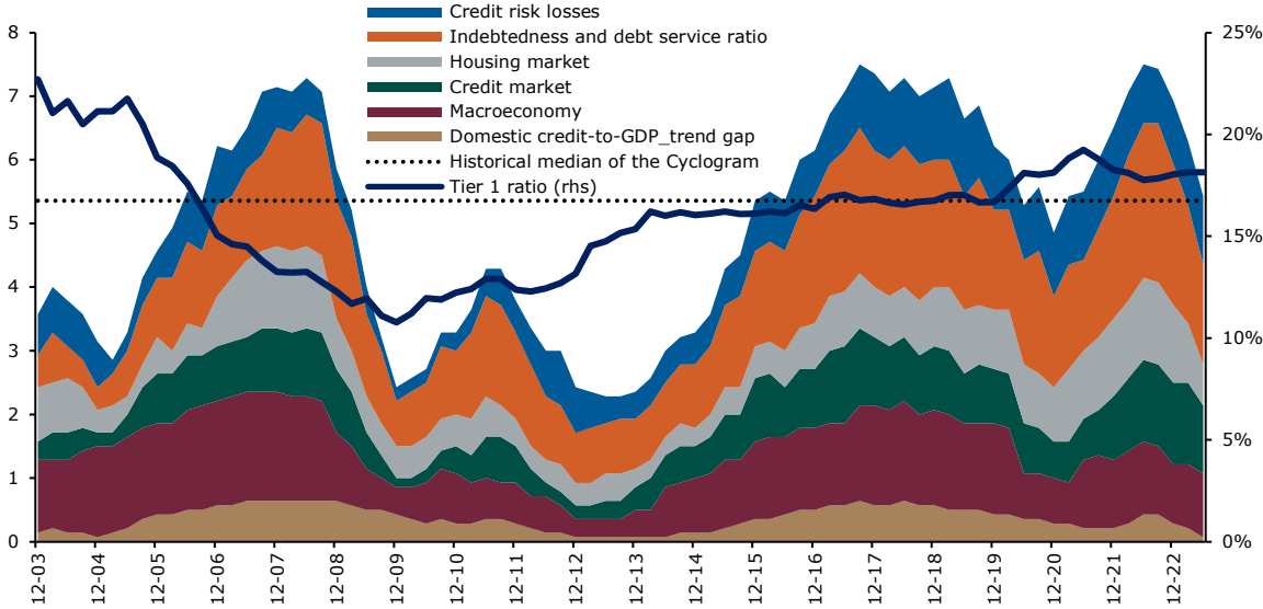
Chart 1 Cyclogram
