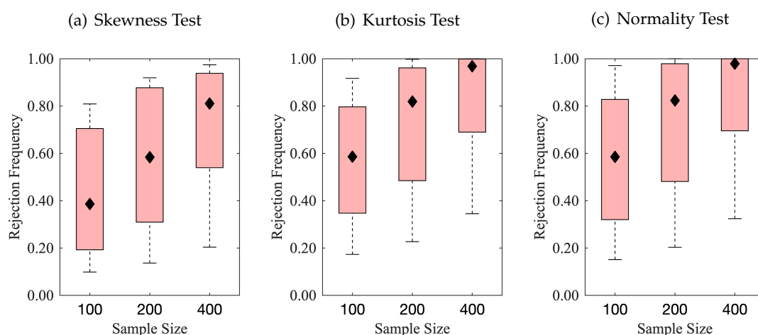
Figure 4: Observed Power of Tests (Non-studentized Statistics)
