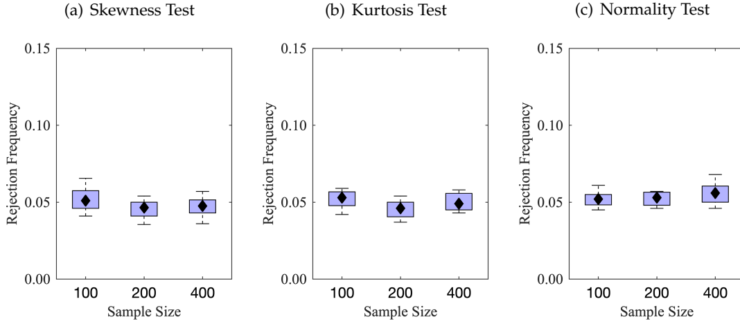
Figure 1: Observed Level of Tests (Studentized Statistics)
