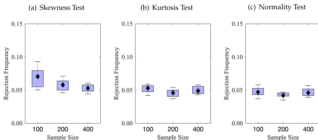
Figure 4: Observed Power of Tests (Non-studentized Statistics)
