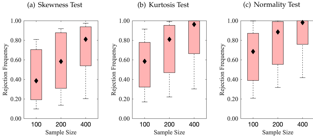
Figure 2: Observed Power of Tests (Studentized Statistics)
