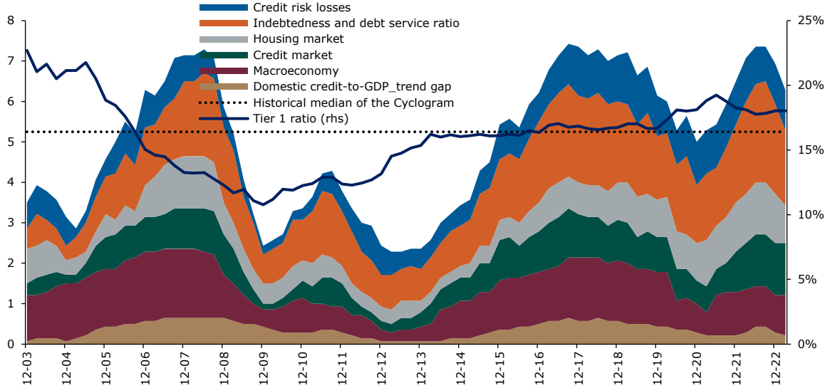
Chart 1 Cyclogram
