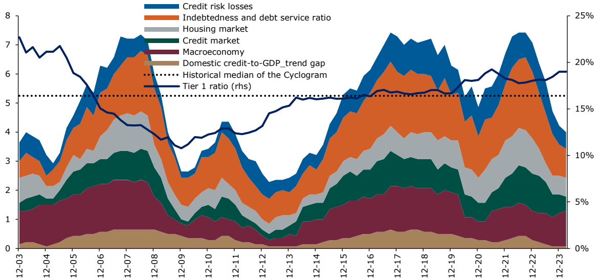
Chart 1 Cyclogram
